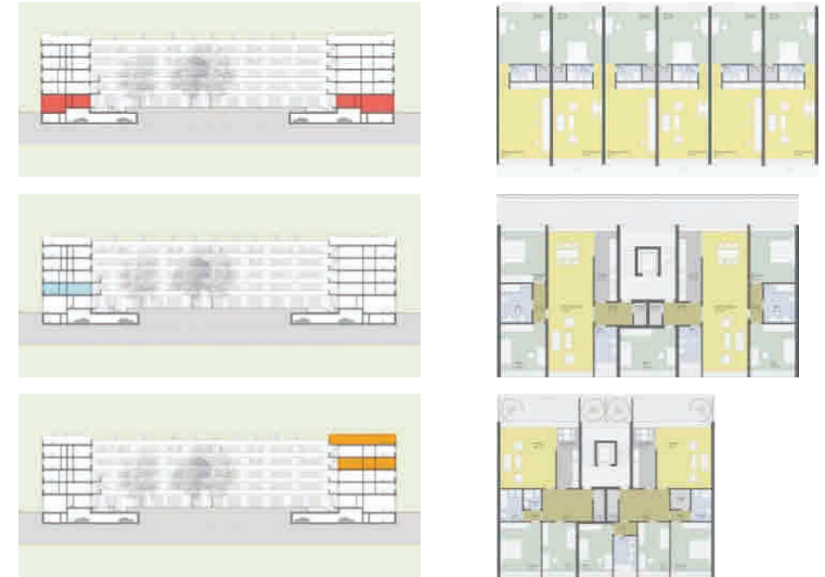
Section and typical apartment © http://dienerdiener.ch/en/project
